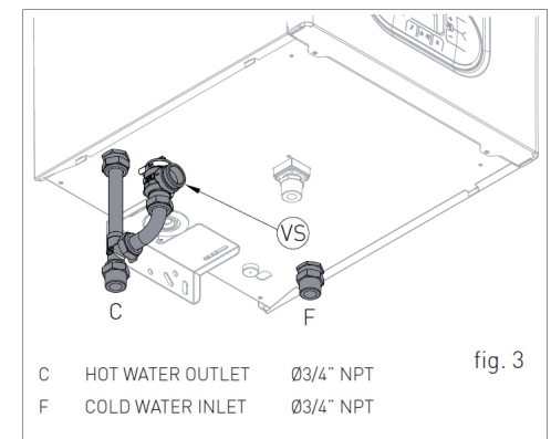
Water connection under SFK 55 models with standard supplied pipe kit.
